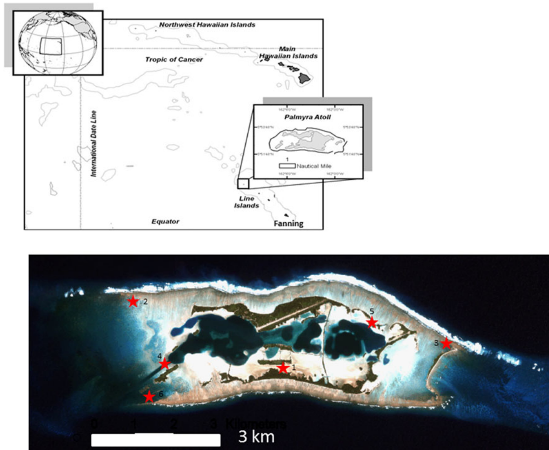
Fig. 1. Map of Palmyra Atoll within the Line Island chain. Red stars display the location of lemon shark sightings or capture. Numbers by stars refer to details in Table 1.
